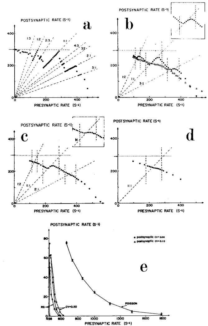
Fig. 1. Mean rate transformation (MRT) for inhibitory synapse. On the abscissa and the ordinate, the corresponding pre- and postsynaptic rates over a stationary period. The paradoxical segments are determined with regular trains in each case and their slopes and bounds are indicated by broken lines. The spontaneous postsynaptic rate without IPSP's is indicated by a dotted horizontal line. Different graphs correspond to different pre- or postsynaptic discharge irregularities measured by the interval coefficient of variation (CV). a. Regular pre- and postsynaptic trains. Several paradoxical segments are visible. A presynaptic rate above 470/s silenced the postsynaptic firing. b. Presynaptic interval CV 0.10; Postsynaptic CV 0.03 (circles), 0.10 (asterisks for 1:1 in inset) or 0.35 (triangles). c. Presynaptic CV 0.20; Postsynaptic CV 0.00 (circles) or 0.10 (inset for 1:1 PS). d. Presynaptic CV 0.30. e. High presynaptic rates: Presynaptic train regular or irregular with CV 0.20 or 1.00 (Poisson); Postsynaptic CV 0.00 (circles) and 0.10 (triangles).
