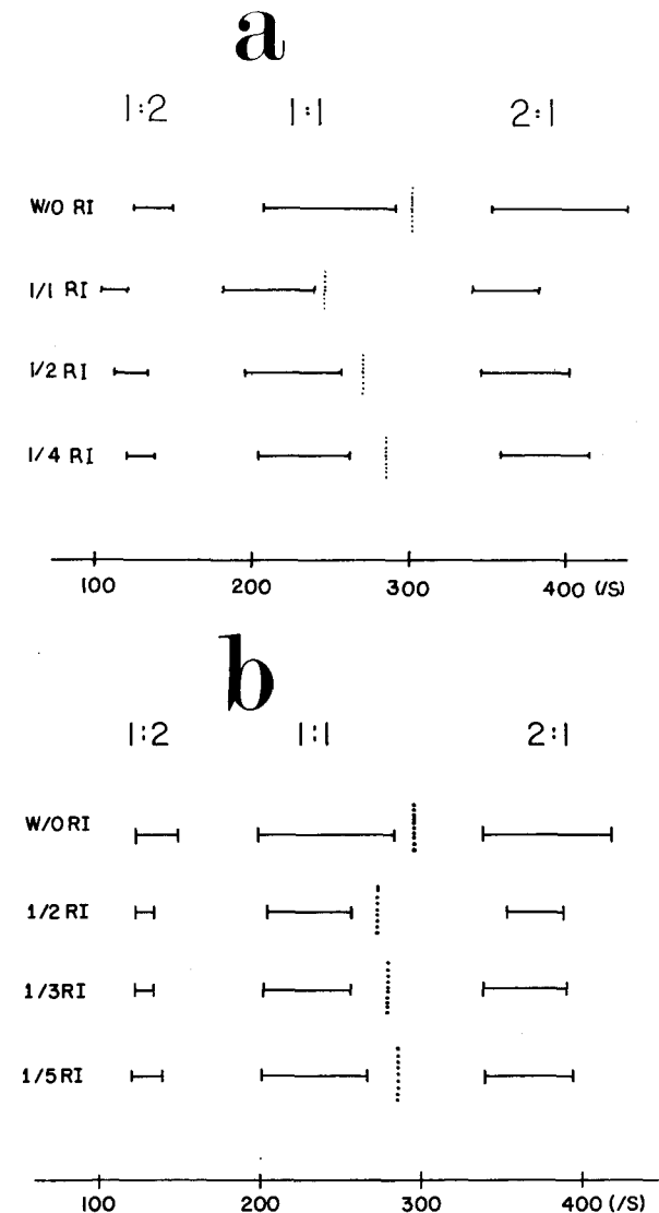
Fig. 2. Locking ranges for (a) deterministic and (b) pseudo-random recurrent inhibition (RI) for different feedback ratios 1/k . The horizontal scale is the rate of the regular external presynaptic train. The upper sequence of 3 horizontal bars indicates the ranges where 1:2, 1:1 and 2:1 PS's occurred without RI. The vertical dotted lines are the respective postsynaptic spontaneous rates, higher for no RI than with RI. The spontaneous rates with no RI are different for (a) and (b) because of circuit details.
