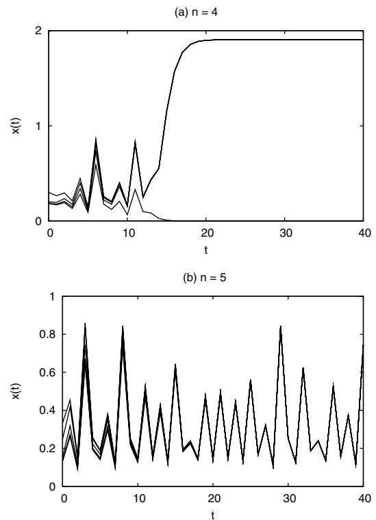
Fig. 3: Dynamics of all-to-all coupled leaky neurons starting from random initial conditions. The 4-neuron system (a) does not synchronize, but the dynamics remain simple, whereas the 5-neuron system (b) synchronizes, and the synchronous solution is chaotic. The parameter values are as in fig. 2.
