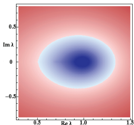
Fig. 5: The mixed transverse exponent \chi as a function of \lambda for the dynamics (21) and the parameter values \alpha = 100, \beta = 20, \epsilon = -1 . Blue indicates negative values of \chi and red positive values, respectively.
